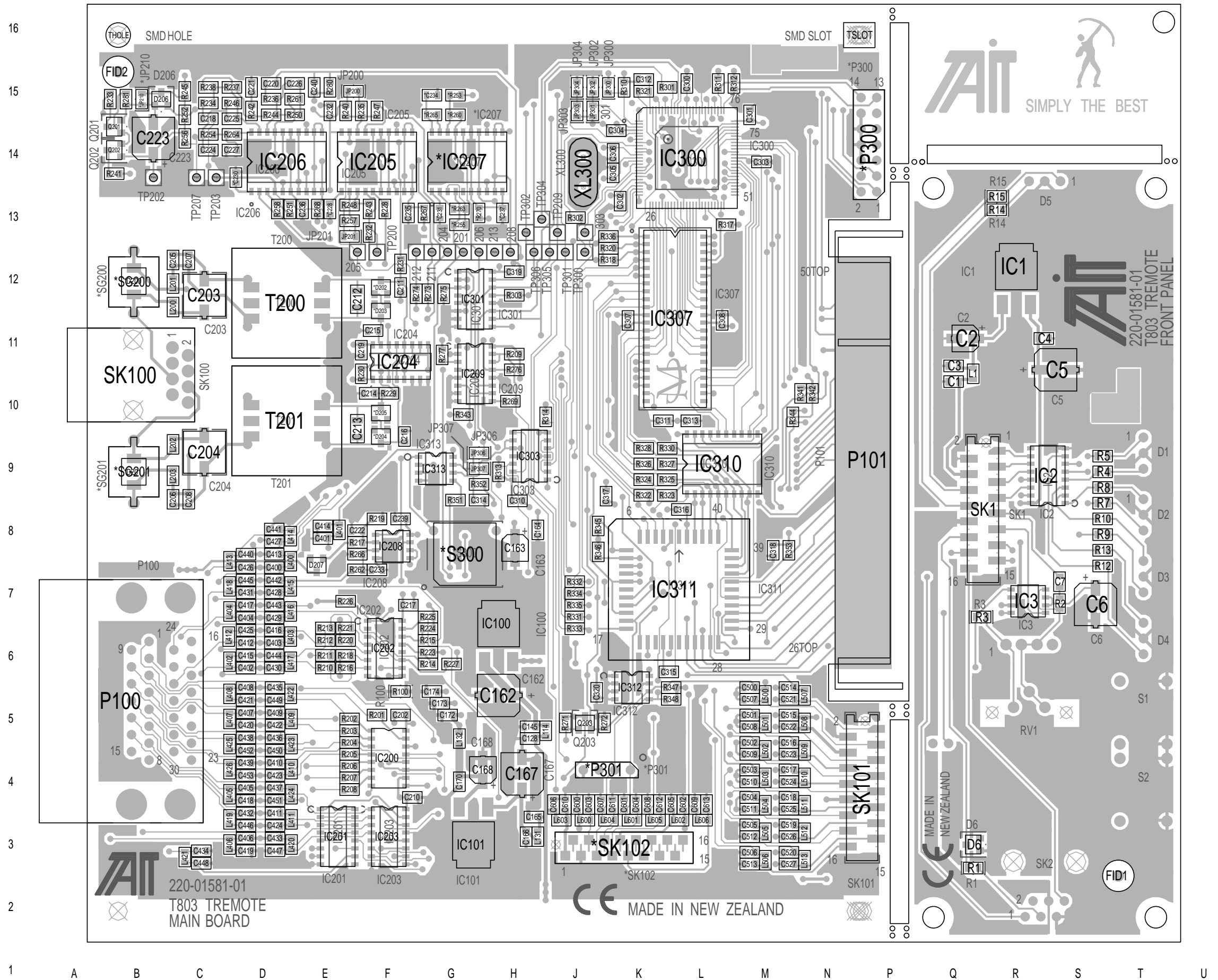
T803 PCB Layout - Top Side 220-01581-01
