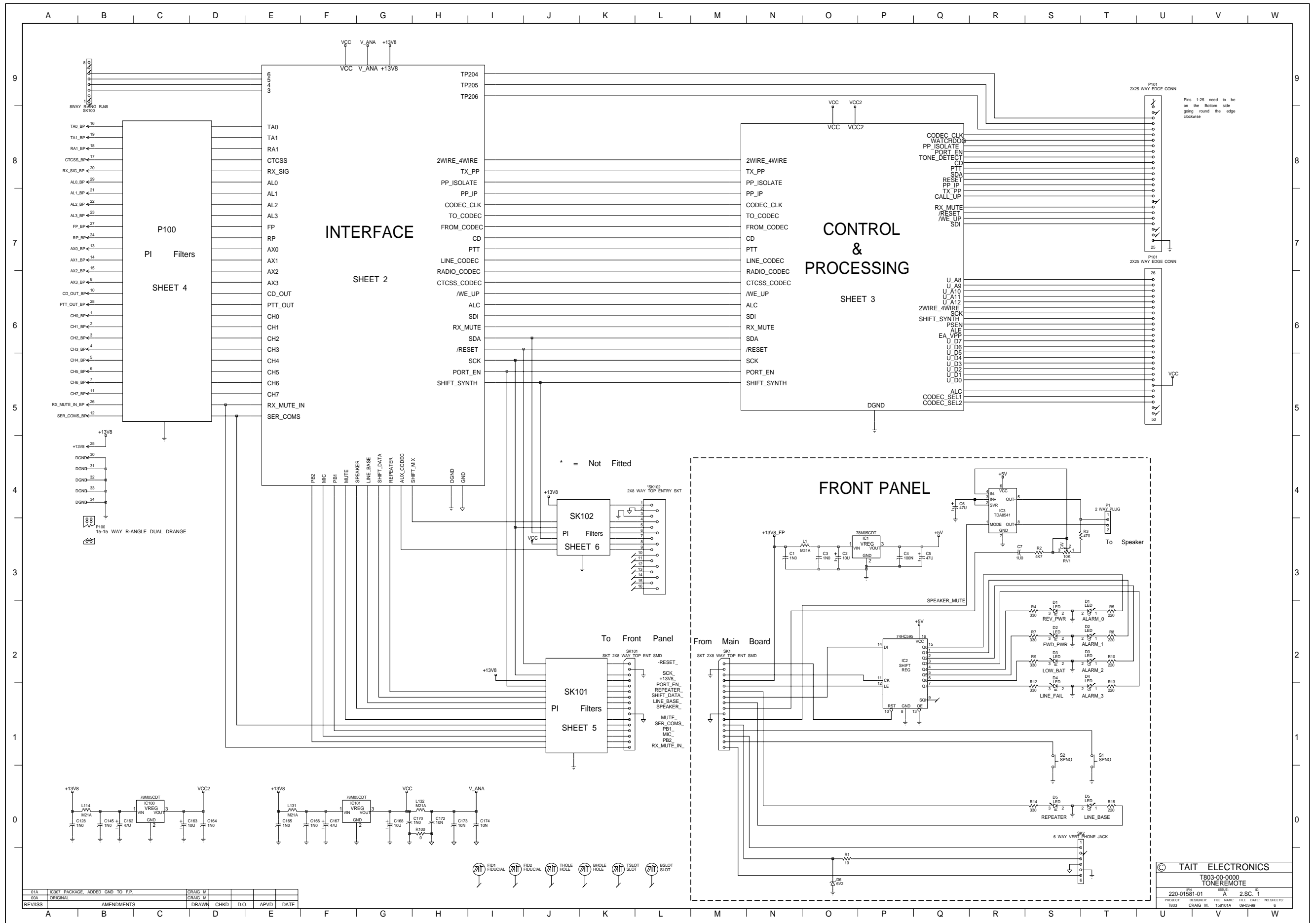
Sheet 1 - T803 Overview & Front Panel 220-01581-01
