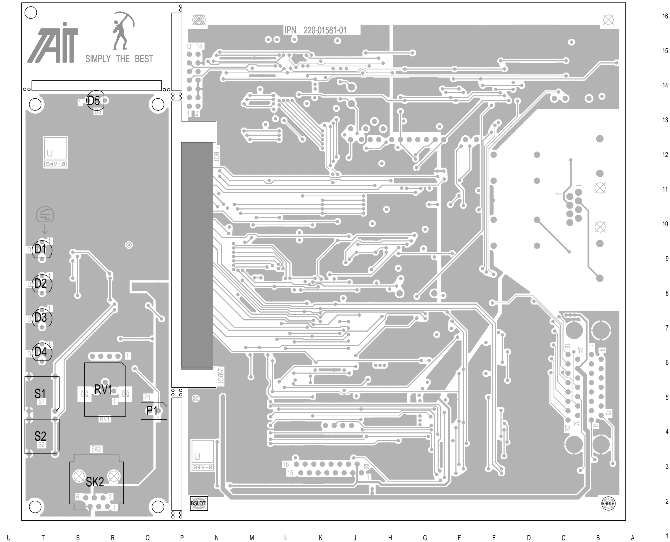
T803 PCB Layout - Bottom Side 220-01581-01
